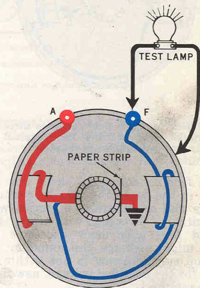
Figure 8—Check for grounded motor-generator.
